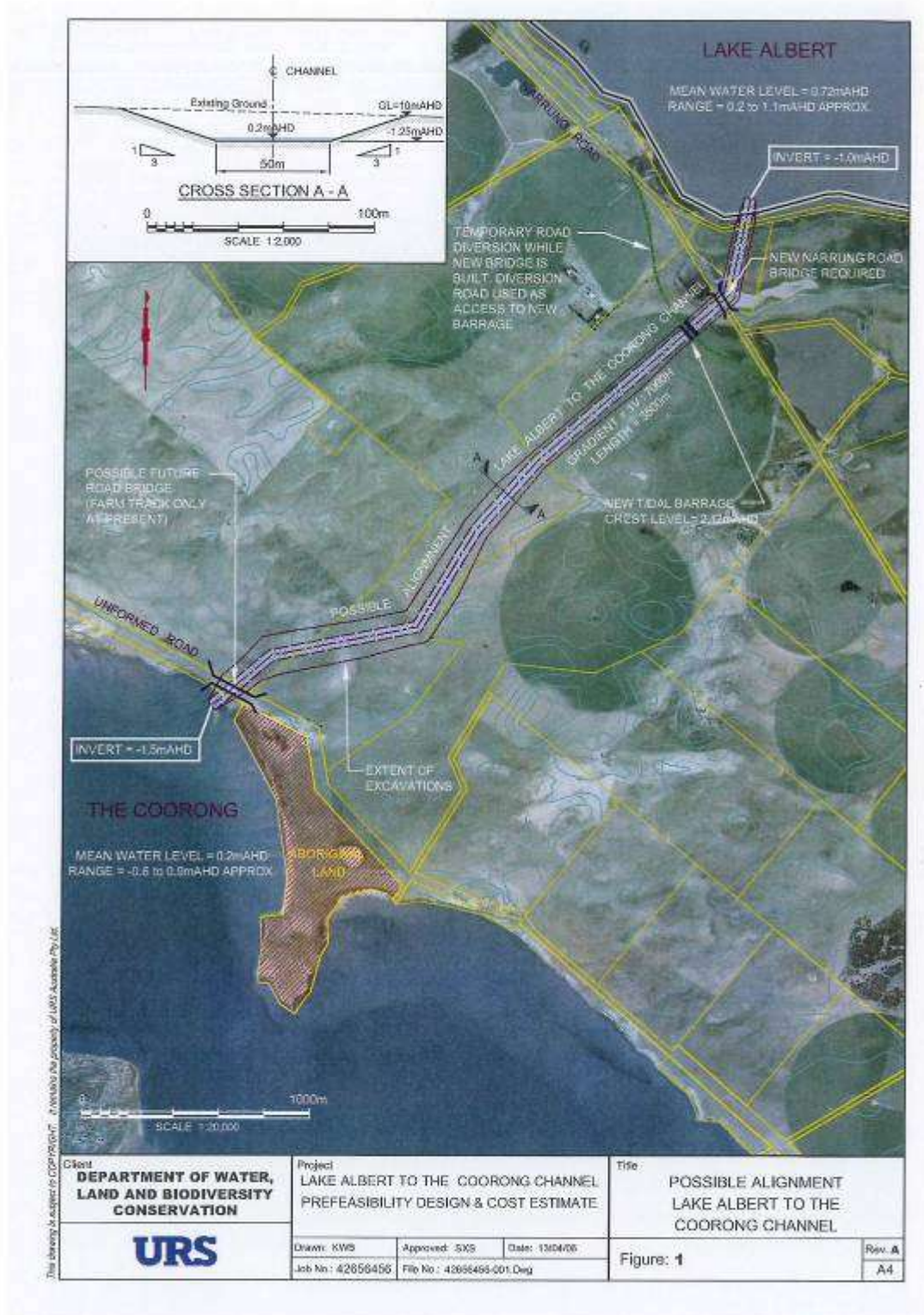
Figure 11: URS (2006) pre-feasibility concept design drawing
